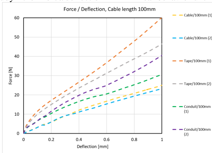
Figure 6. Experimental Force/Deflection responses for a high-voltage cable length of 100 mm and various covers.
